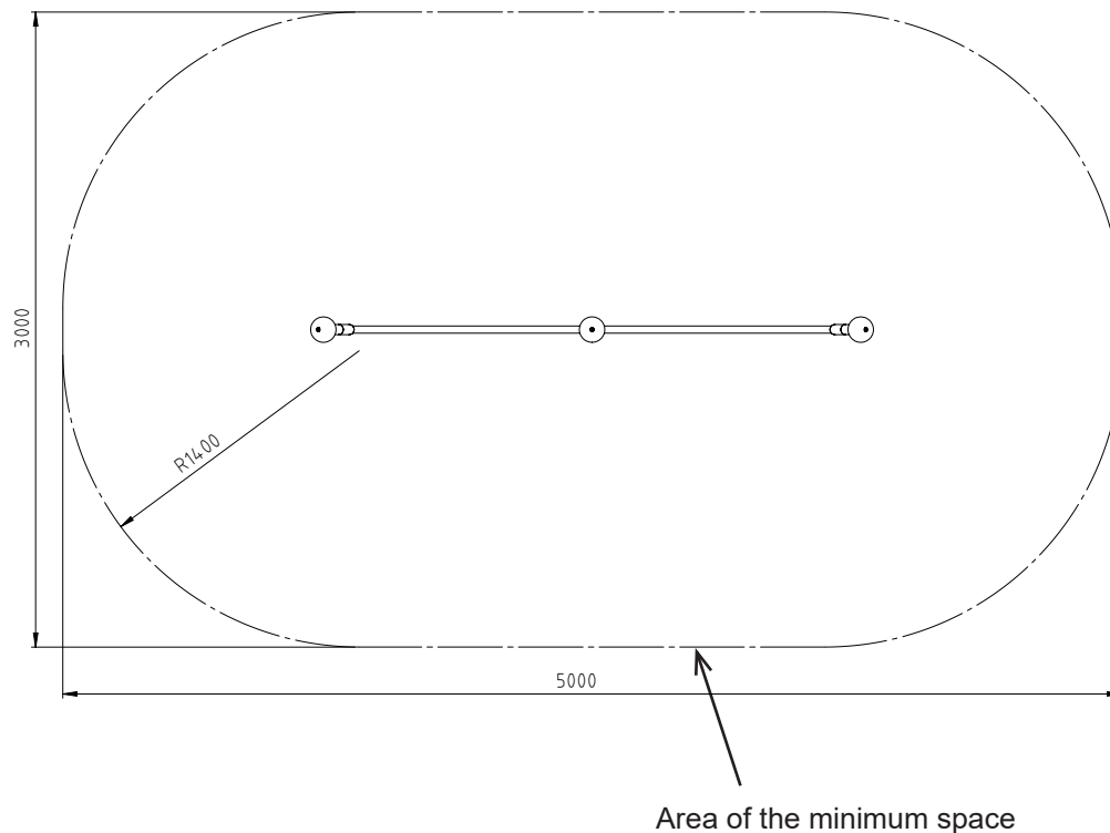
Diagram 3: Top view
